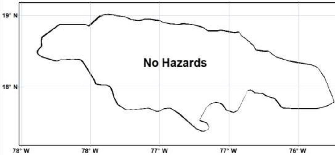
Week-2 Jamaica Heat Hazard Outlooks Valid: 05 - 11 Feb 2025
