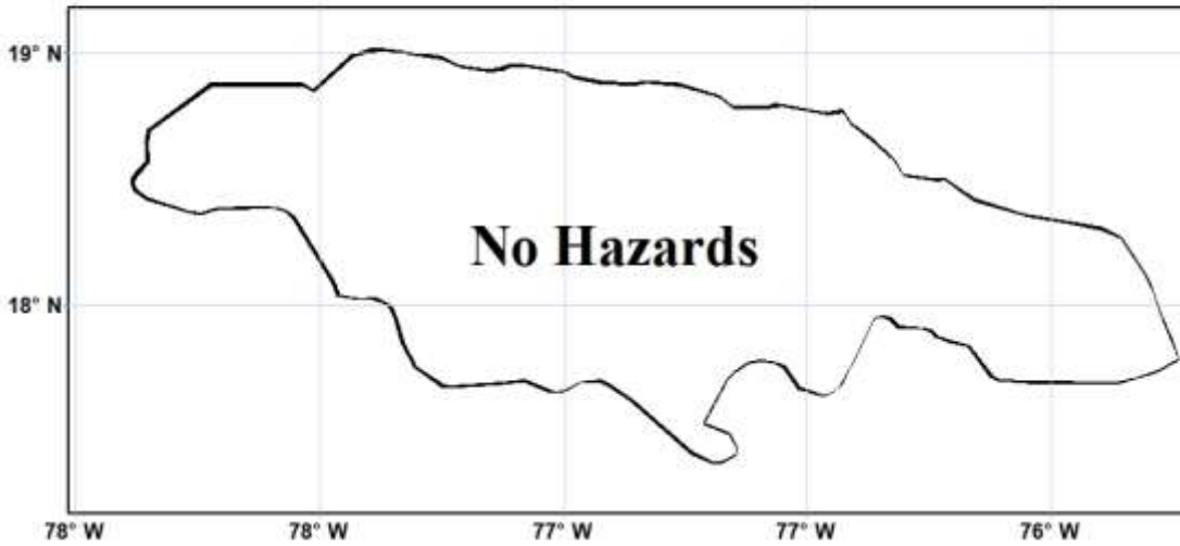
Week-1 Jamaica Heat Hazard Outlooks Valid: 29 Jan - 04 Feb 2025
